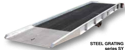
13 1/2" USABLE LIP SUPPORT EDGE FITS INTO TRAILER OR BUILDING SAFETY CHAINS STANDARD
